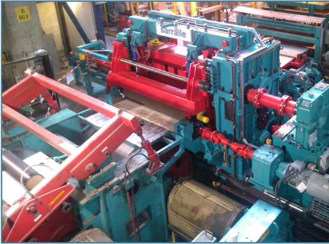
Process line productivity increase: Replacement of a hydraulic shear for a heavy duty 7mm rotary shear.
